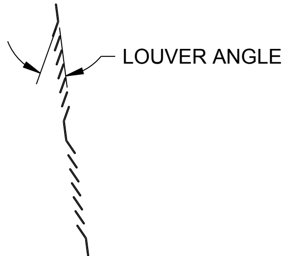
SECTION A-A CROSS SECTION OF FIN GEOMETRY, PER TUBE ROW
